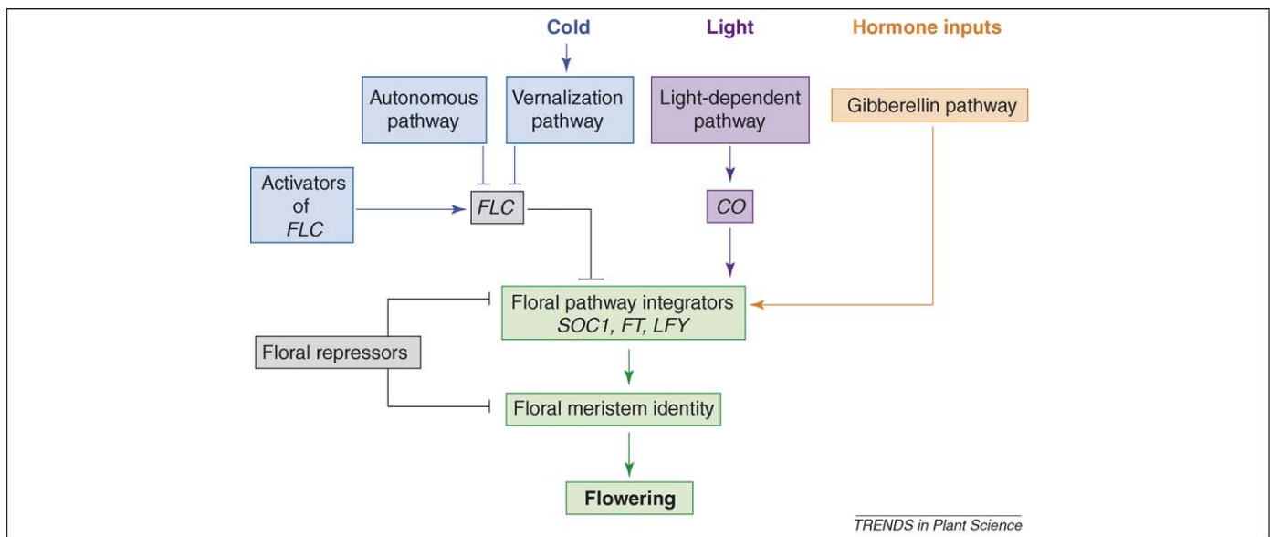
Figure 1. Interacting flowering time genetic pathways. Although complex interactions occur among the different flowering-time genetic pathways (See Ref. [9] for example), we have intentionally simplified the overall network of flowering-time regulation for a better understanding. Abbreviations: CO , CONSTANS ; FLC , FLOWERING LOCUS C ; FT , FLOWERING TIME ; LFY , LEAFY ; SOC1 , SUPPRESSOR OF OVEREXPRESSION OF CONSTANS .
